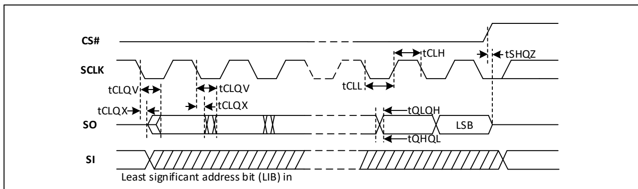
Figure-48. Output Timing
