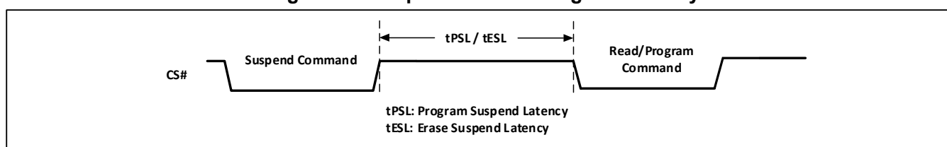
Figure-38. Suspend to Read/Program Latency
