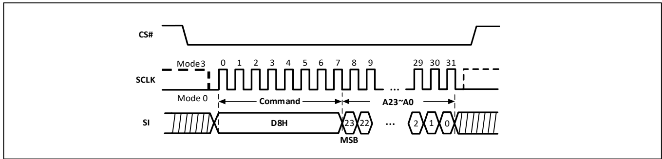
Figure-33. Block Erase Sequence Diagram
