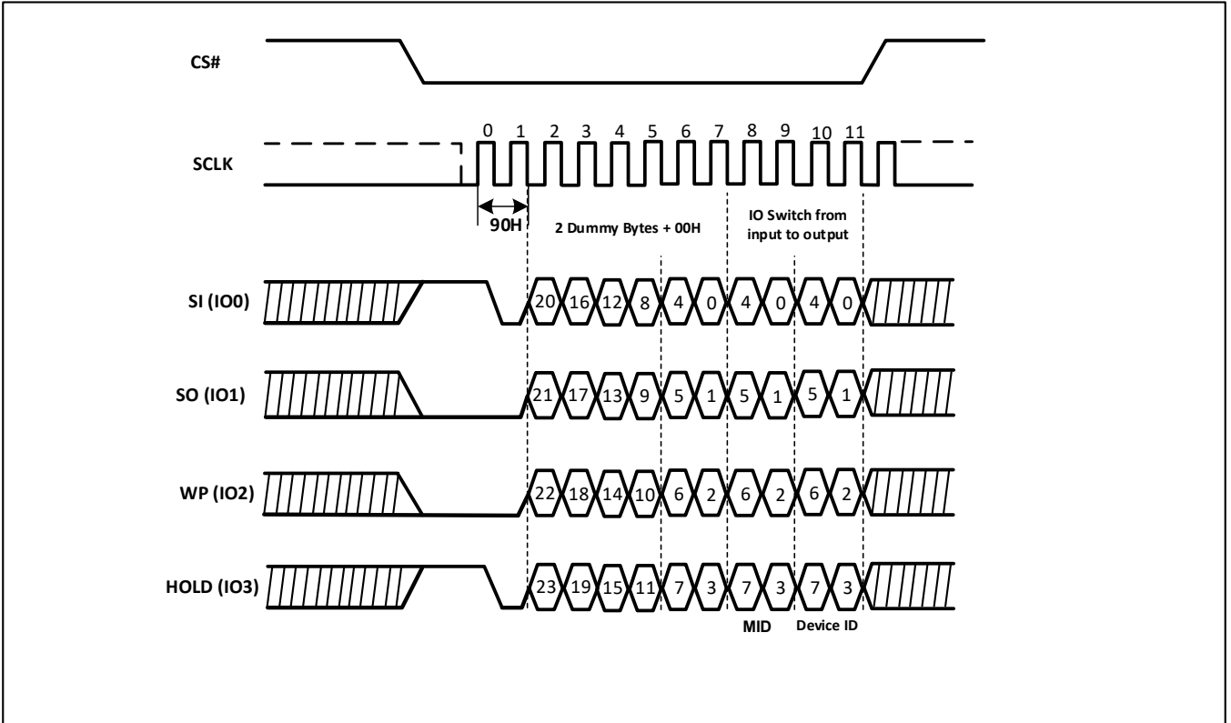
Figure-58. Read Electronic Manufacturer ID & Device ID Sequence Diagram (QPI)
