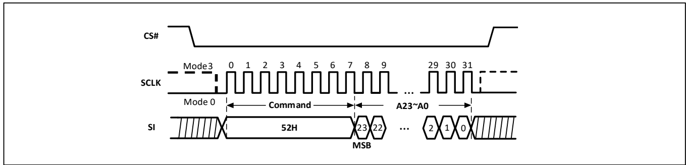
Figure-31. Half Block Erase Sequence Diagram
