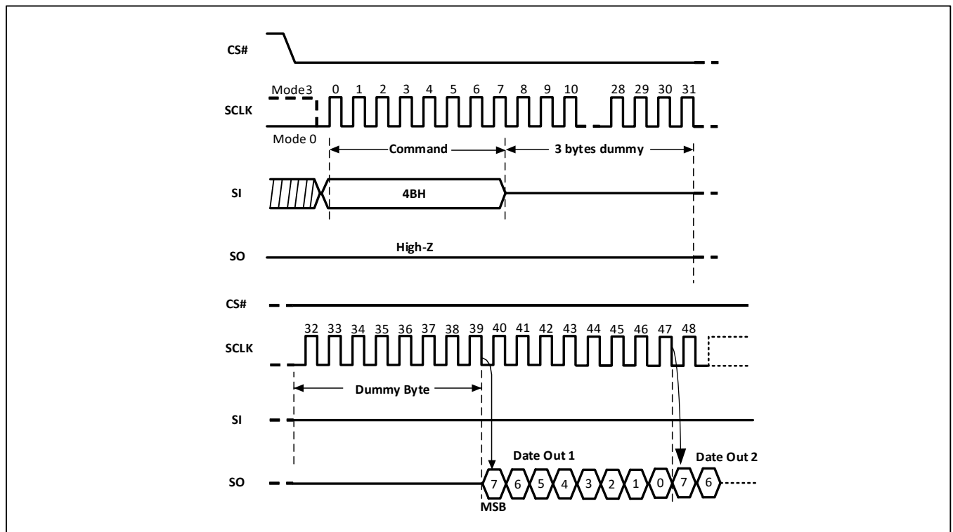
Figure-68. Read Unique ID Sequence Diagram
