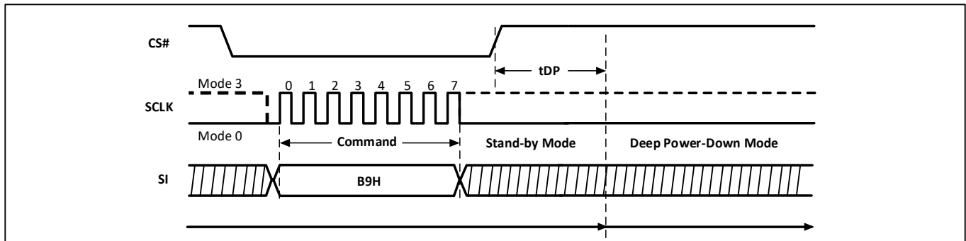
Figure-30. Deep Power-Down Sequence Diagram
