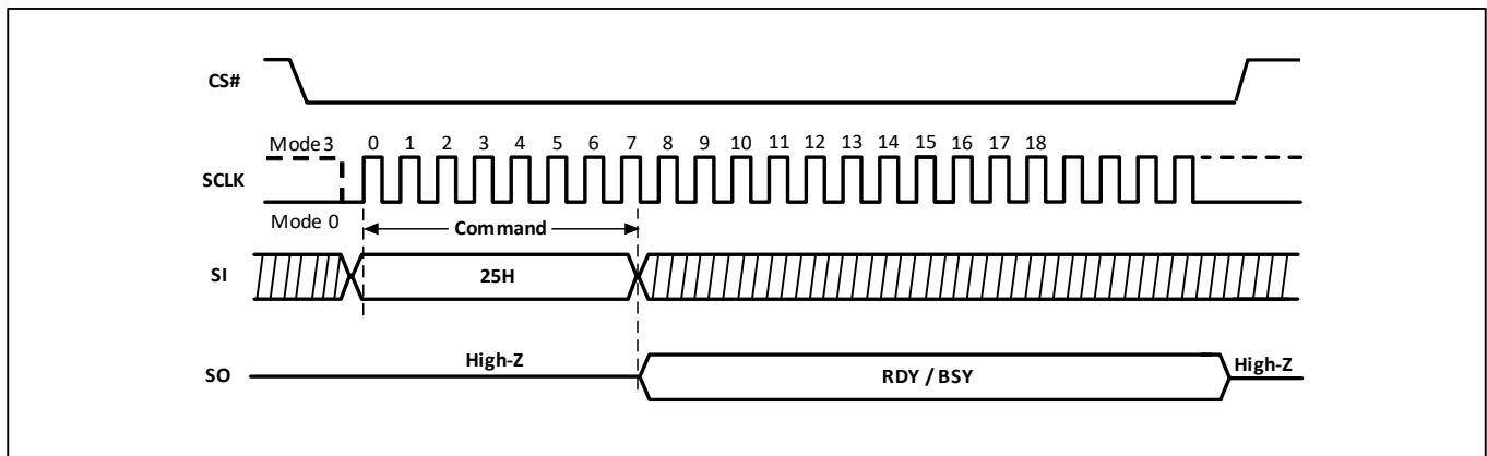
Figure-7. Active Status Interrupt Sequence Diagram
