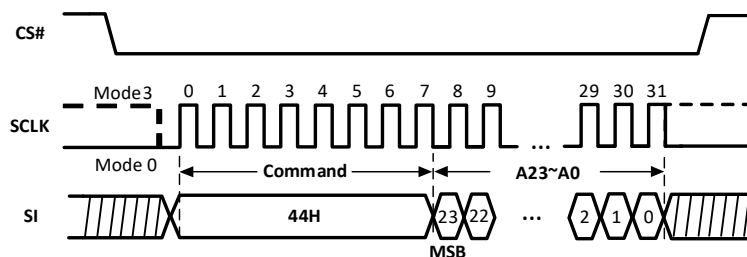
Figure-41. Erase Security Register Sequence Diagram
