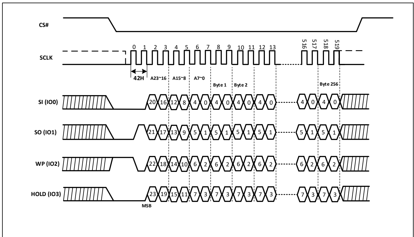
Figure-44. Program Security Register Sequence Diagram(QPI)
