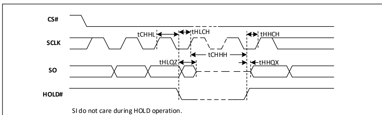
Figure-80. Hold Timing
