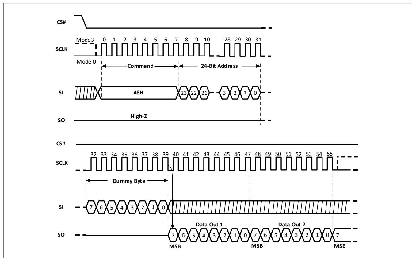
Figure-45. Read Security Register Sequence Diagram
