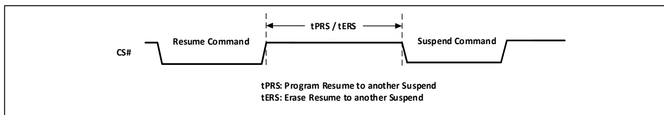
Figure-63. Resume to Suspend Latency
