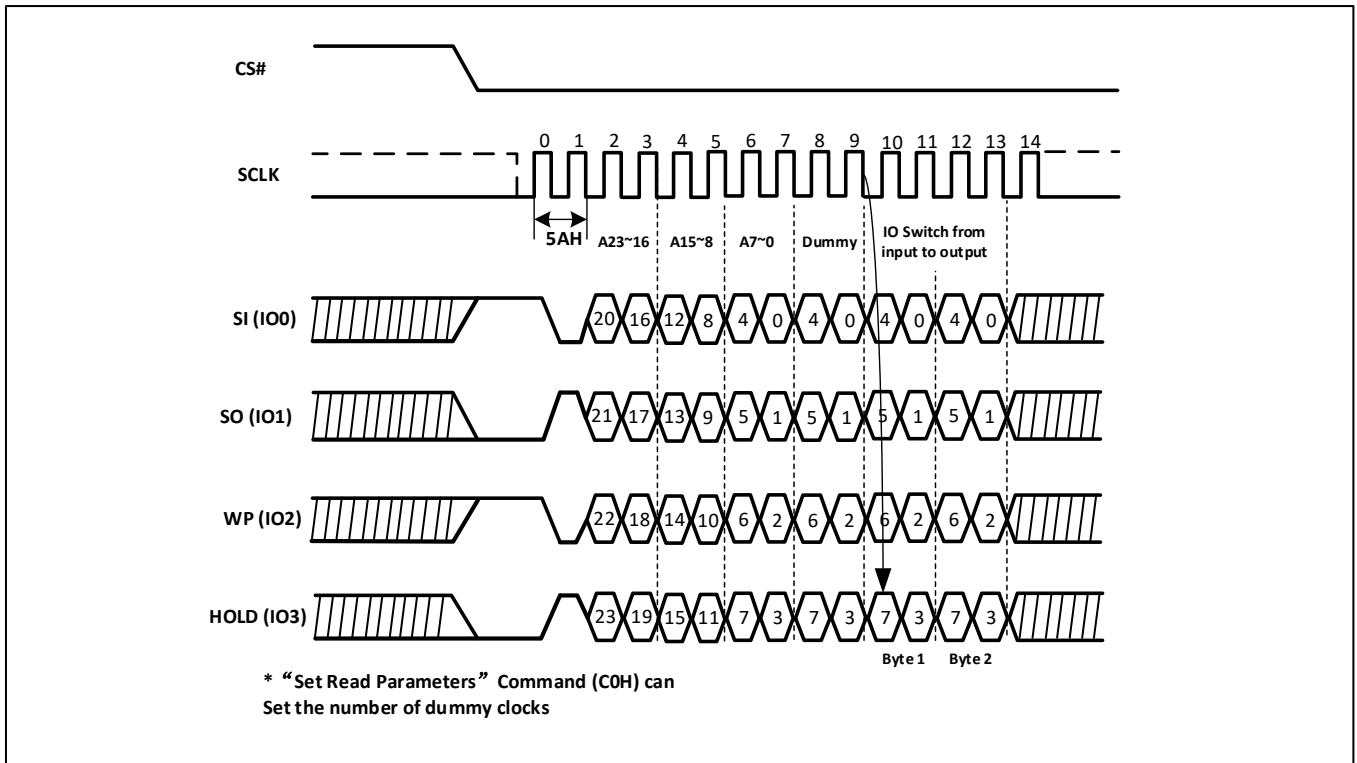
Figure-70. Read Serial Flash Discoverable Parameter Sequence Diagram (QPI)
