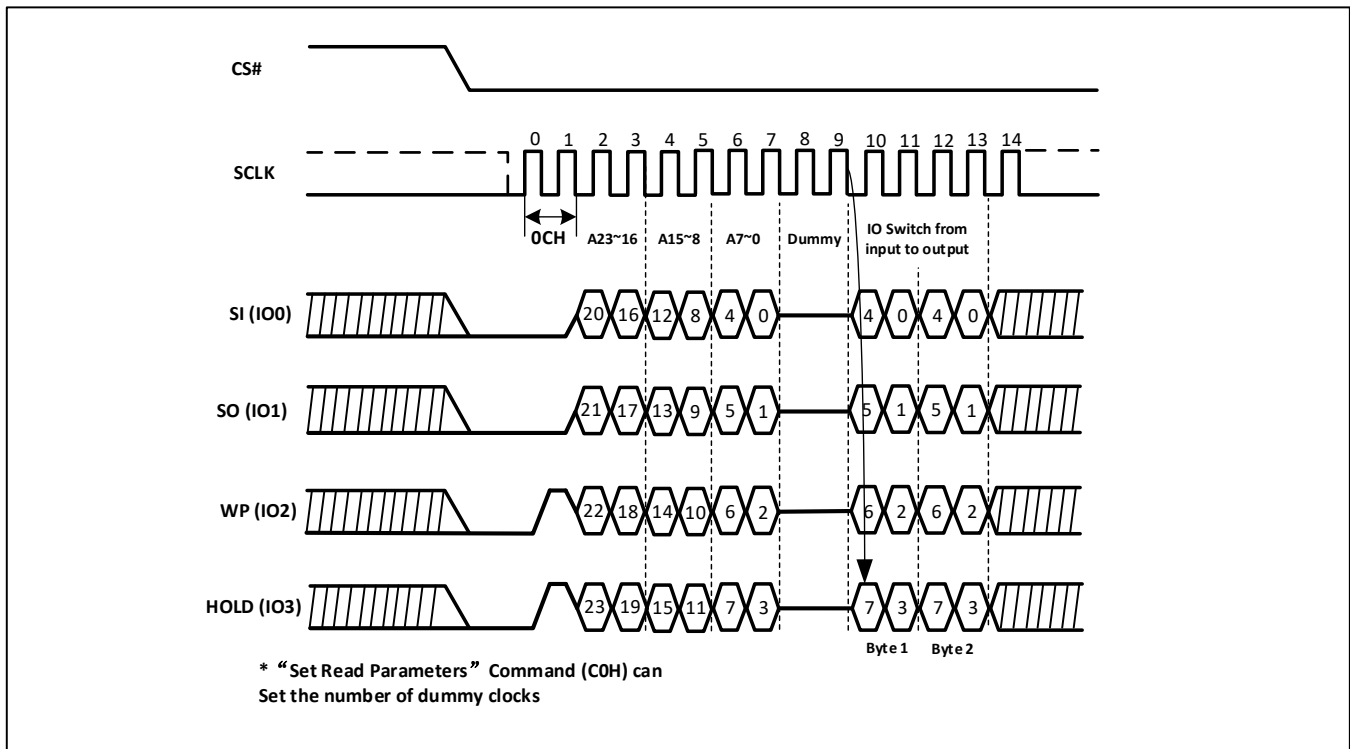
Figure-25. Burst Read with Wrap Sequence ( QPI )
