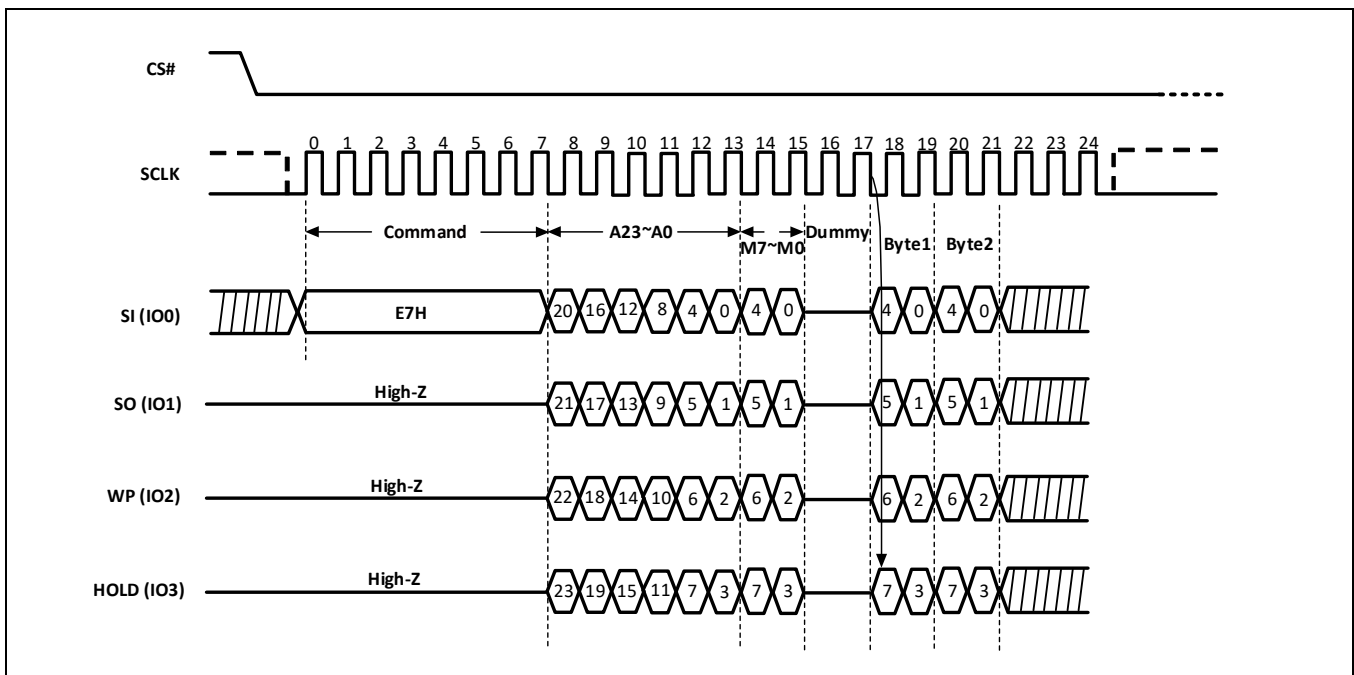
Figure-22. Quad I/O Word Read Sequence (M5-4 ≠ (1,0))
