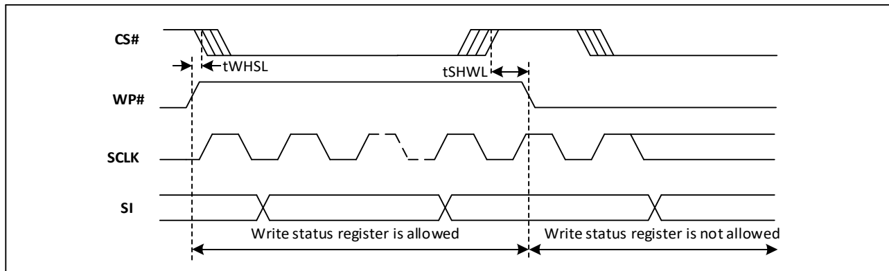
Figure-81. WP Timing
