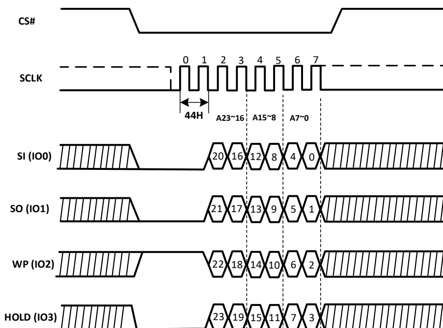
Figure-42. Erase Security Register Sequence Diagram (QPI)
