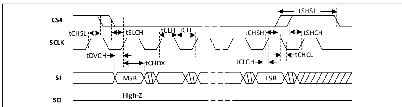
Figure-85. Serial Input Timing
