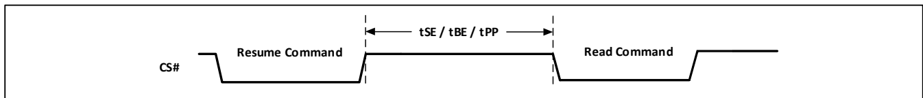
Figure-72. Program Resume and Erase Resume Sequence Diagram
