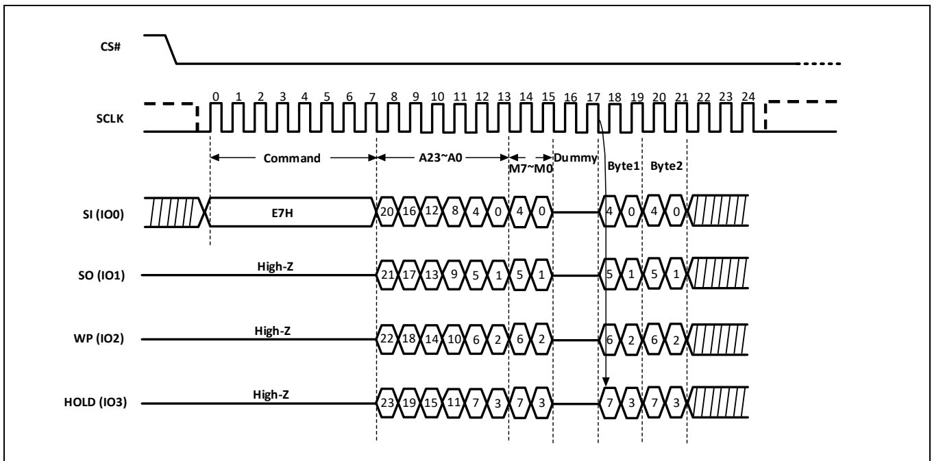
Figure-24. Quad I/O Word Read Sequence (M5-4 ≠ (1,0))
