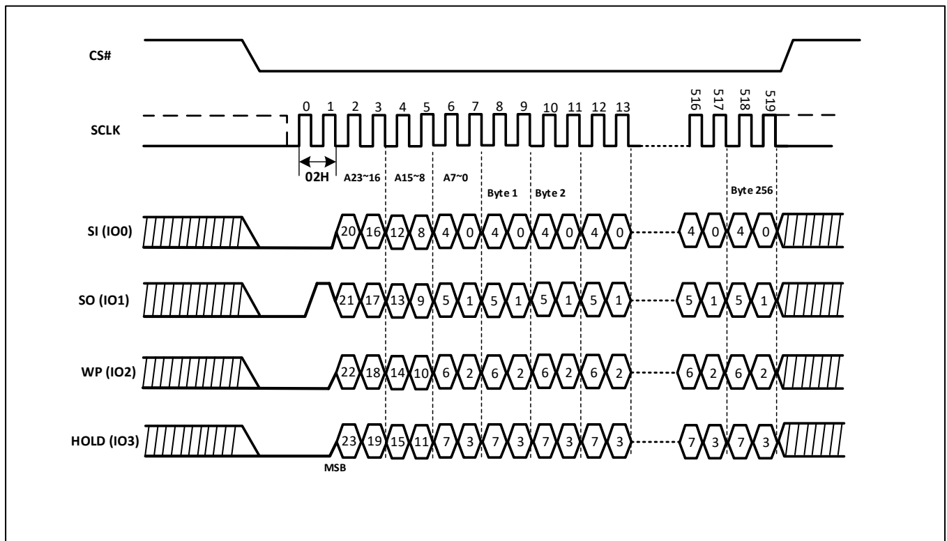
Figure-42. Page Program Sequence Diagram (QPI)
