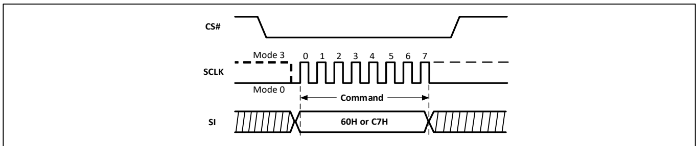
Figure-39. Chip Erase Sequence Diagram
