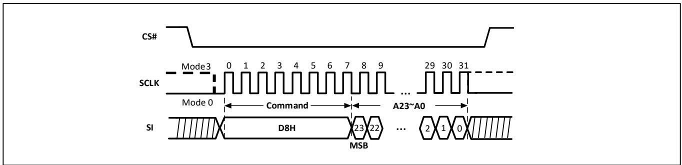
Figure-37. Block Erase Sequence Diagram
