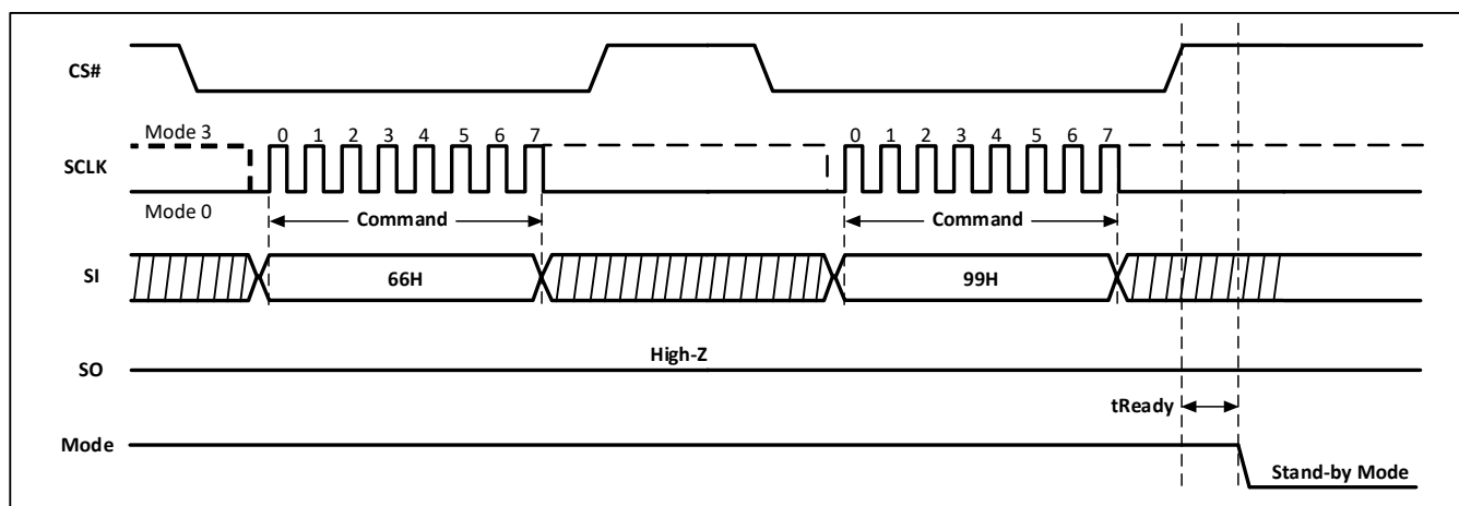
Figure-67. Reset Enable and Reset Sequence Diagram
